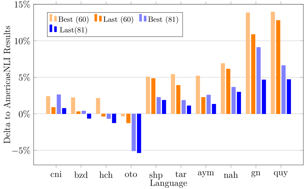
Figure 4.3: Difference between our achieved performance and the reported performance in Ebrahimi et al. [2022]. Lower is better. The languages are ordered by amount of data available in ascending order.
